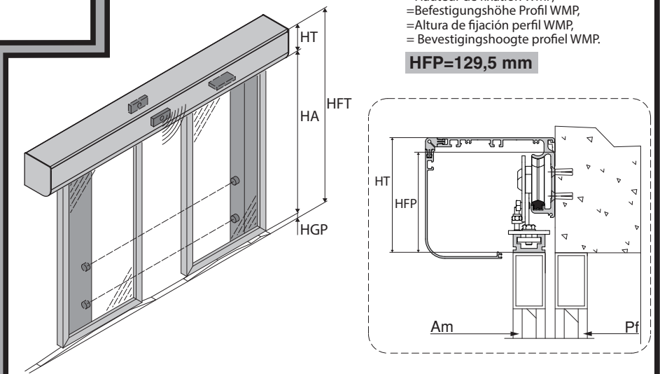
Vista SL 107 - 125: Destra, Right, Droitea, Rechts, Derecha, Rechts.
